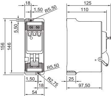
8562/52-..., 1-pole + N
