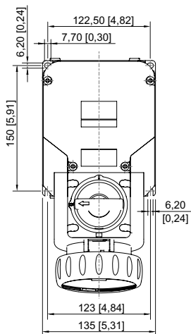
Wall-mounting socket
