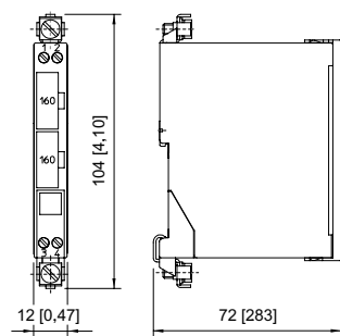
Single-Channel Safety Barriers for Alternating Polarity
