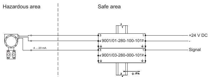
Application: 3-wire 4 ... 20 mA transmitter
