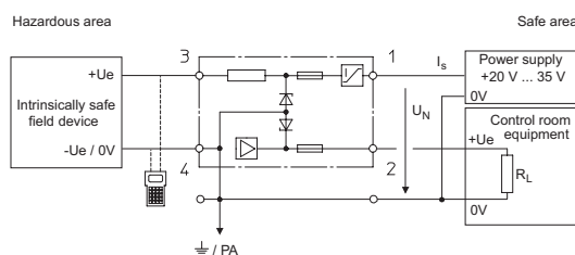
Single-Channel Safety Barriers for Transmitters
