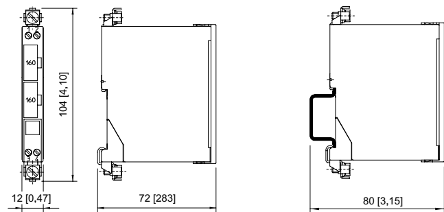
mounted on the NS 35/15 mounting rail
