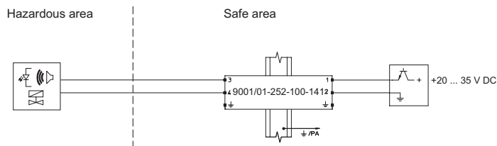
Single-Channel Safety Barriers for Positive Polarity
