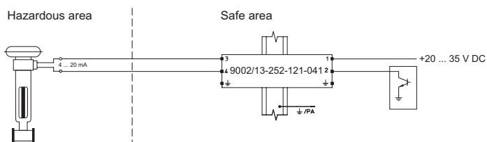
Application: Analogue output (power source) for I/P converters etc., field circuit unearthed
