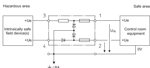
Dual-channel safety barrier, safety barrier potential: + / evaluation barrier potential: +
