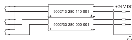
Application: Combination of potential-free contacts
