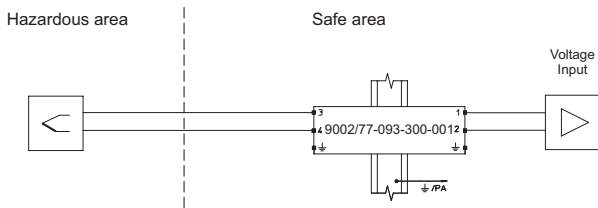
Application: Thermocouples
