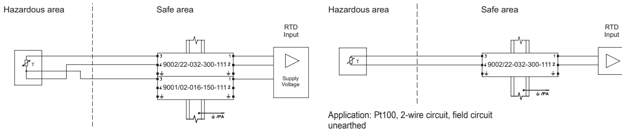
Application: Pt100, 3-wire circuit, field circuit unearthed
