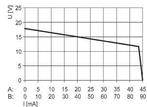
9175/0-14-11, 9176/0-14-00 output characteristic
