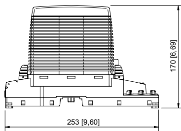
CPU & power module for Zone 1 with connection by means of an unconnected cable end
