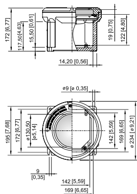
Enclosure size 3 with inspection window
