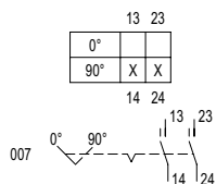
Switching arrangement 8006/4-007-00
