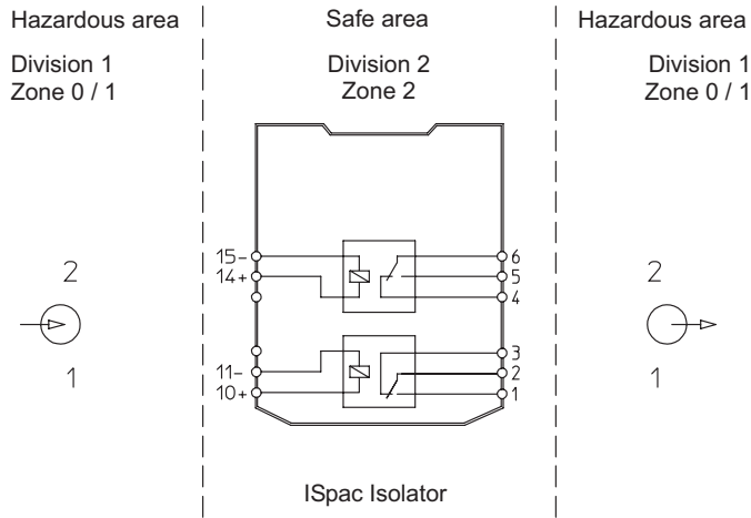
Connection diagram 9172/22-11-00
