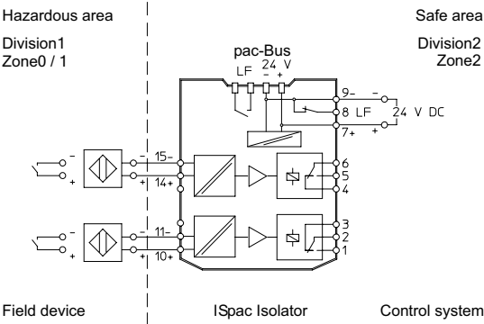
Connection diagram 9170/21-10-11
