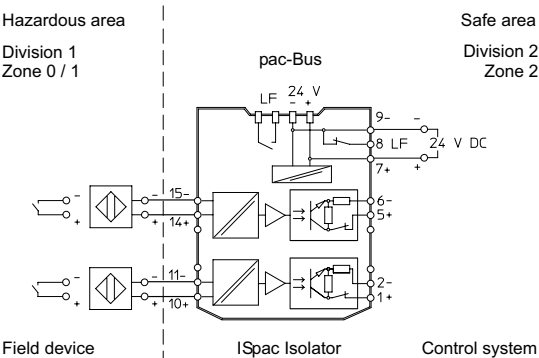
Connection diagram 9170/21-14-12
