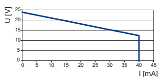
9475/32-04-22 output characteristic
