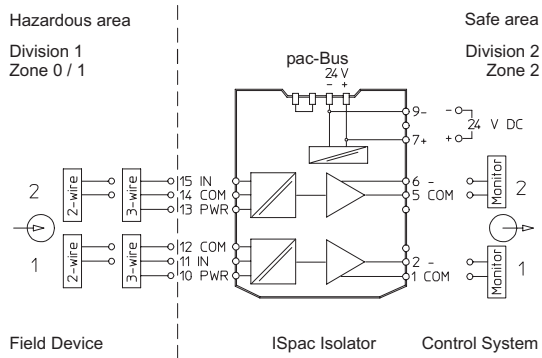
Connection diagram 9147/20-99-10
