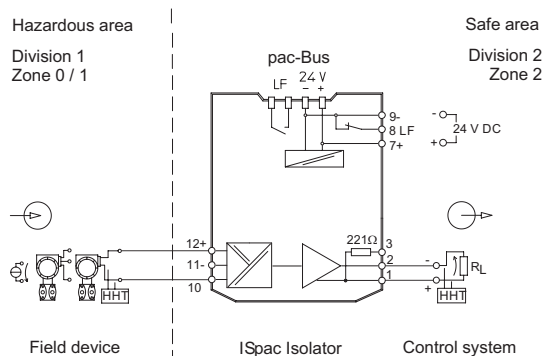
Connection diagram 9160/13-11-11
