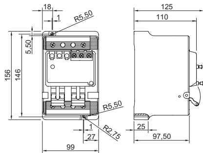
8562/54-2376-060, 2-pole with auxiliary contact and reset function
