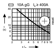
Adjustment range: 2.2 - 3.2 A
