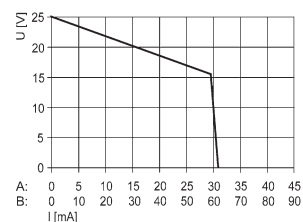
9176/0-15-00 output characteristic
