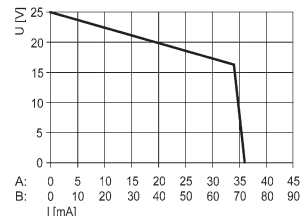
9175/0-16-11; 9176/0-16-00 output characteristic
