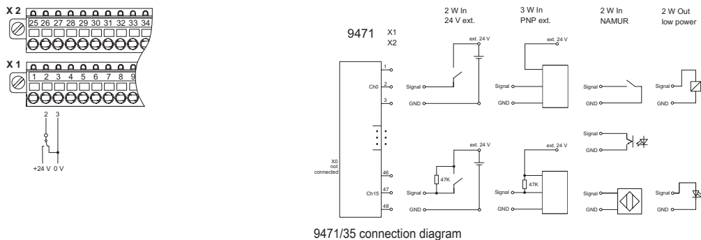
9471/35 connection diagram
