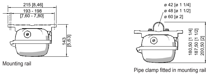
Mounting rail
