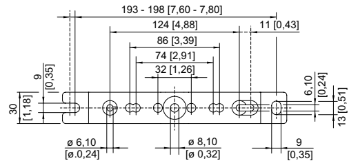
Mounting rail
