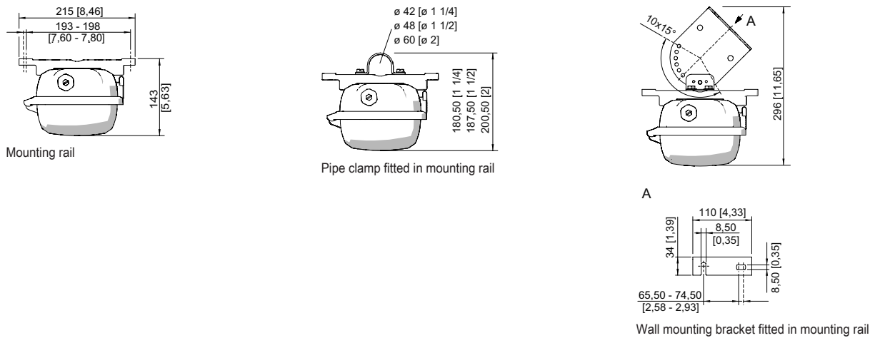
Wall mounting bracket fitted in mounting rail
