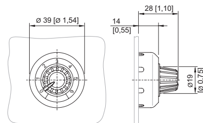
8602/3-092 potentiometer bezel Actuator with radial actuation
