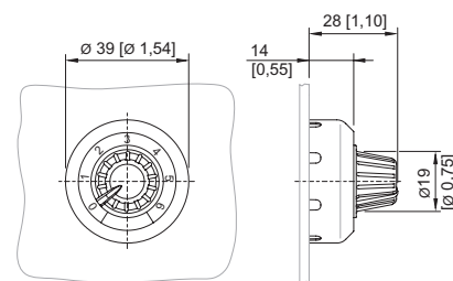
8602/3-092 potentiometer bezel Actuator with radial actuation
