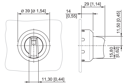
8602/3-726 axial rotary actuator, not lockable Actuator with axial actuation
