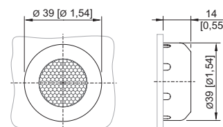
8602/3-735 illuminated pushbutton Actuator with axial actuation
