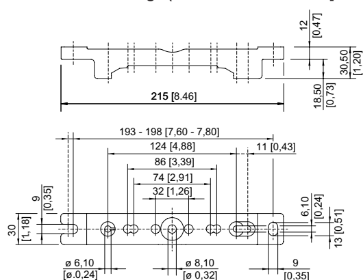
Mounting rail
