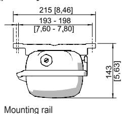
Mounting rail
