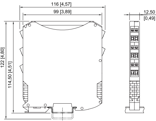
ISpac Series 9260, 9270, 9275, 9276, 9282 with spring clamp terminal
