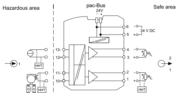
9260/19-11-10 connection diagram
