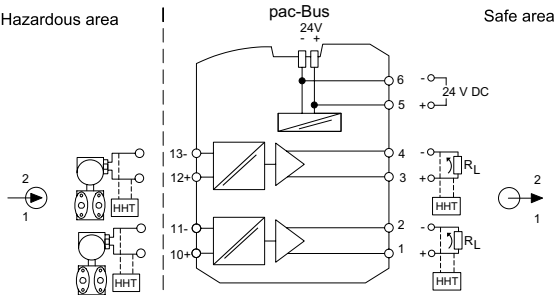
9260/23-11-10 connection diagram
