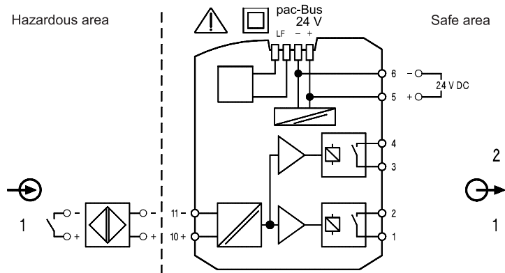
9270/11-17-15 connection diagram
