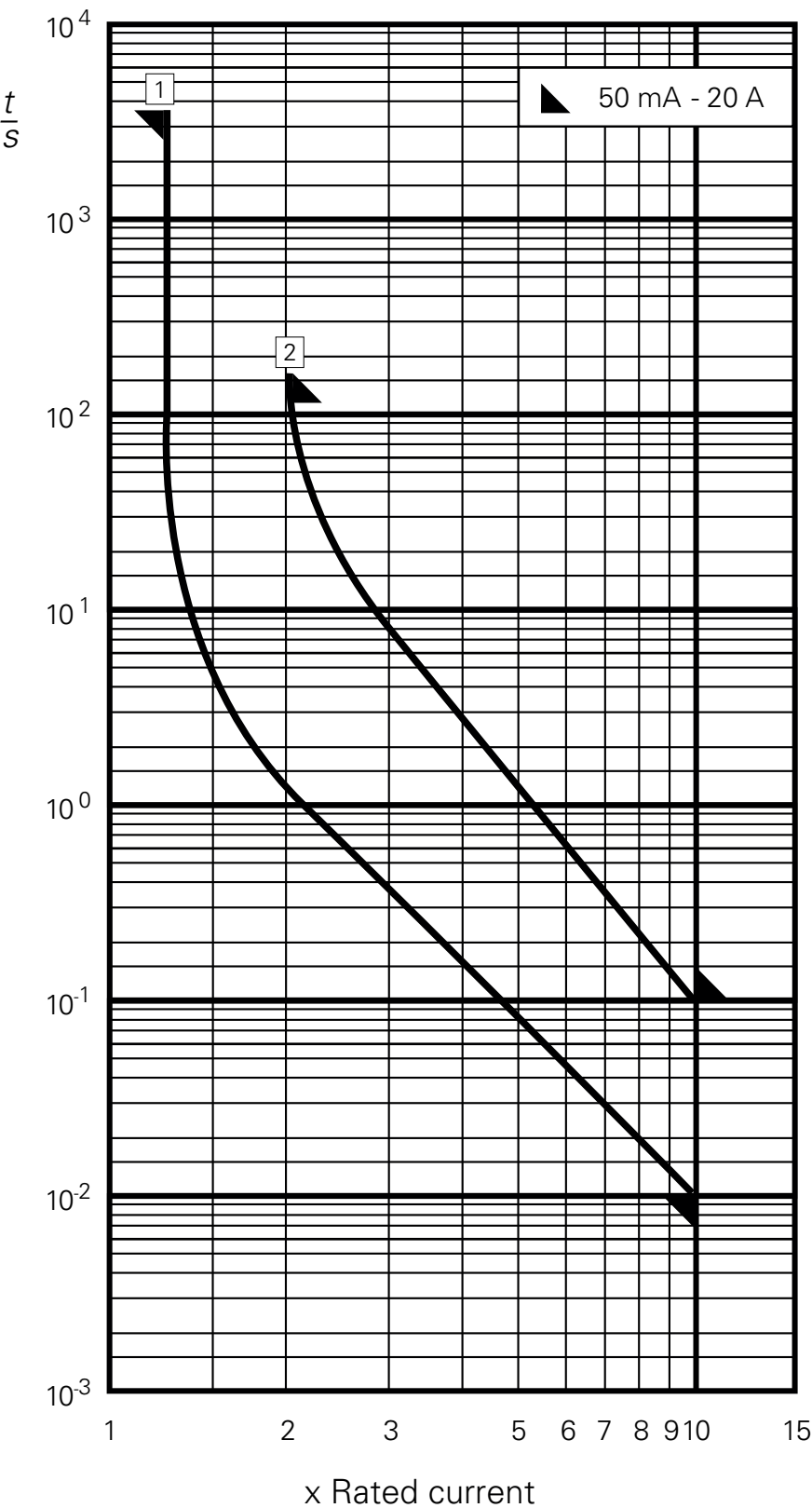
Time-current characteristic 1 = min. tripping time 2 = max. tripping time
