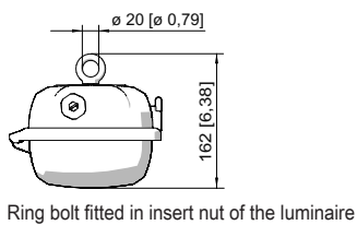
Ring bolt fitted in insert nut of the luminaire
