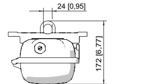
Mounting bracket fitted in mounting rail
