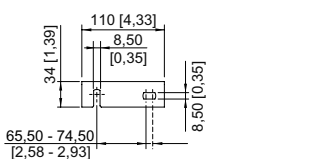
Wall mounting bracket fitted in mounting rail
