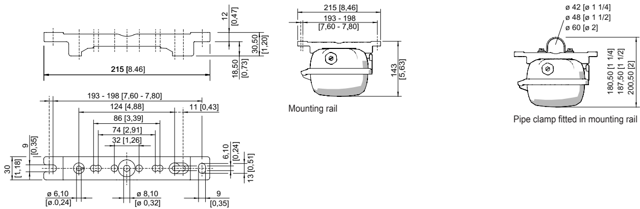
Mounting rail
