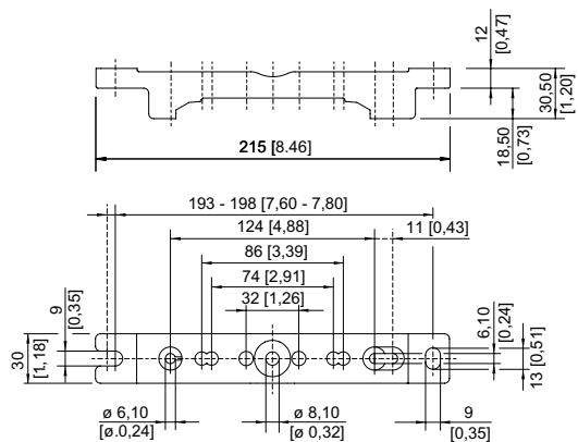
Mounting rail
