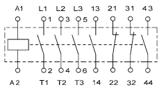
Contact arrangements
