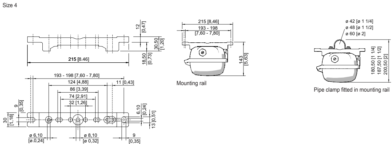
Mounting rail
