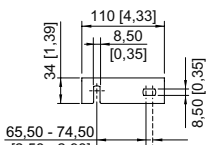
Wall mounting bracket fitted in mounting rail
