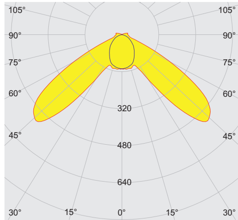
cd/klm — C0 - C180 — C90 - C270 batwing lense
