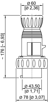
3-pole plug
